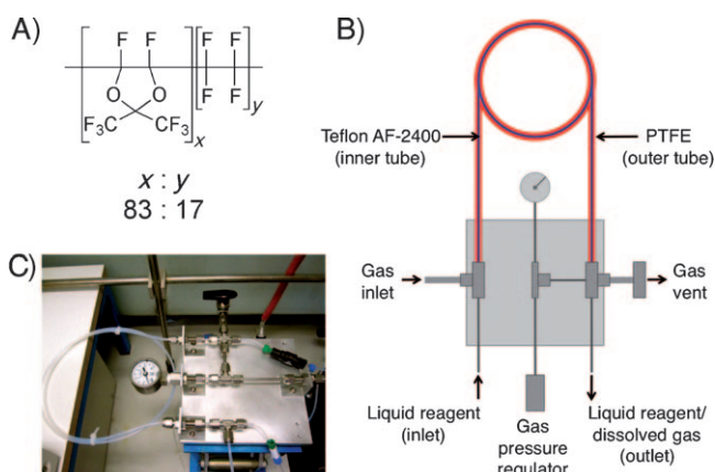
Figure 1. The tube-in-tube flow reactor: A) structure of Teflon AF-2400. B) Schematic of the tube-in-tube reactor configuration (Teflon AF-2400 and PTFE = poly(tetrafluoroethylene)). C) Reactor assembly.
